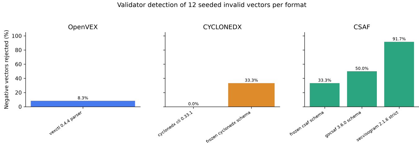
Figure 3. Detection of seeded invalid vectors.
