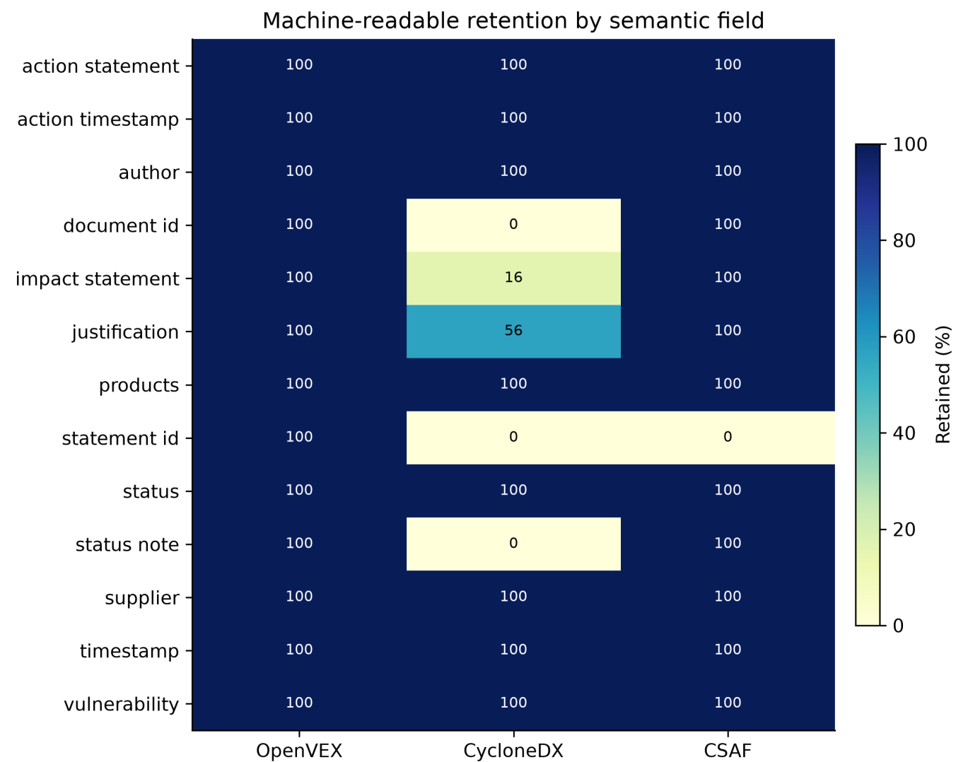
Figure 1. Machine-readable retention by semantic field.
